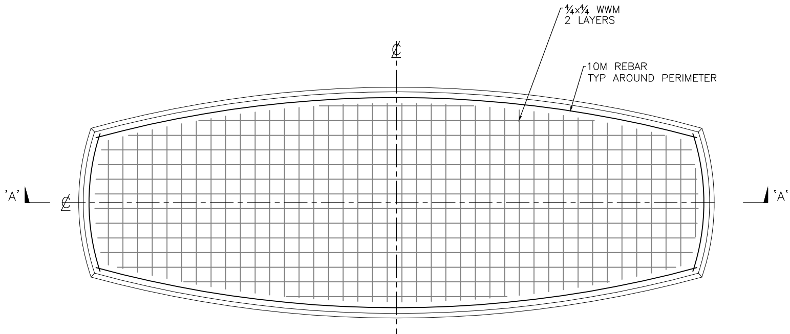
REBAR PLAN
